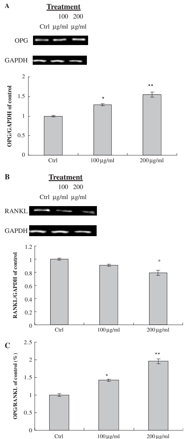
Figure 5. Effect of HEP on OPG and receptor activator of NF- \kappa\text{B} ligand (RANKL) mRNA expression in rat osteoblast-like UMR 106 cells. UMR 106 cells were treated with 100 \mu\text{g ml}^{-1} and 200 \mu\text{g ml}^{-1} HEP extract or its vehicle (ctrl) for 48 h. Total RNA was isolated and subjected to semi-quantitative RT-PCR analysis of OPG (A) and RANKL (B) mRNA expression under the conditions described in 'Methods'. (C) The ratio of OPG/RANKL was normalized by an internal control gene glyceraldehyde-3-phosphate dehydrogenase (GAPDH). Results were obtained from two independent experiments and expressed as mean \pm SEM. *P < 0.05 , **P < 0.01 , versus control for n = 3 .
